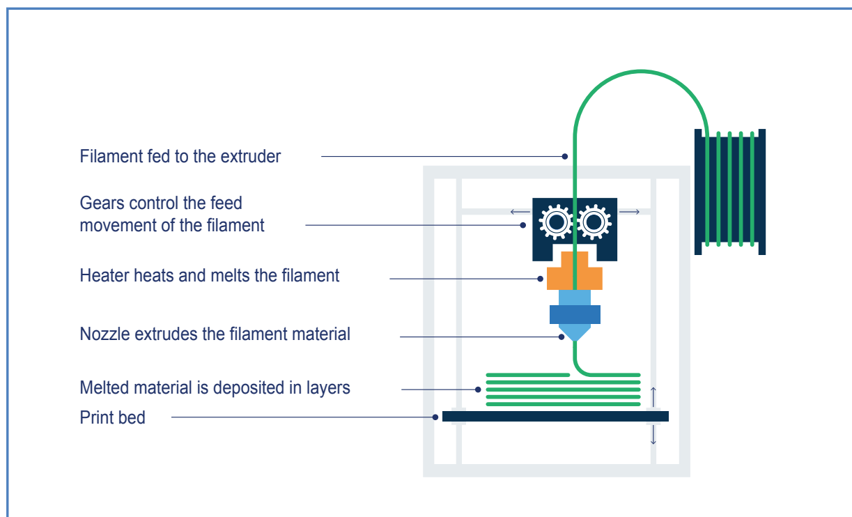
Figure 3 Material Extrusion 3D Printing Process
